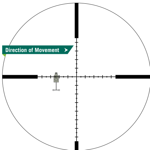
9.5 MOA reticle correction for a target moving 3 mph at a distance of 800 yards. No wind. Elevation already dialed into turret.
