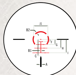
AR-BDC2
