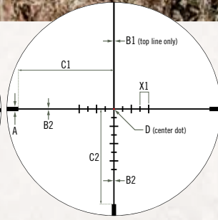
VMR-2 MRAD
